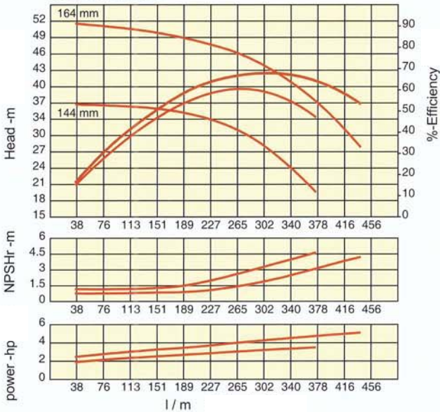
GMP542 60Hz
