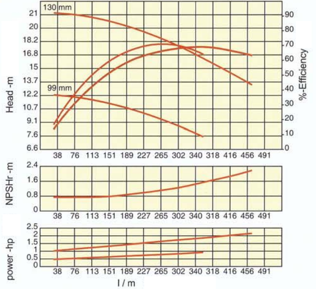
GMP541 50Hz
