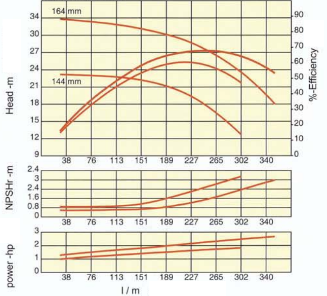
GMP542 50Hz
